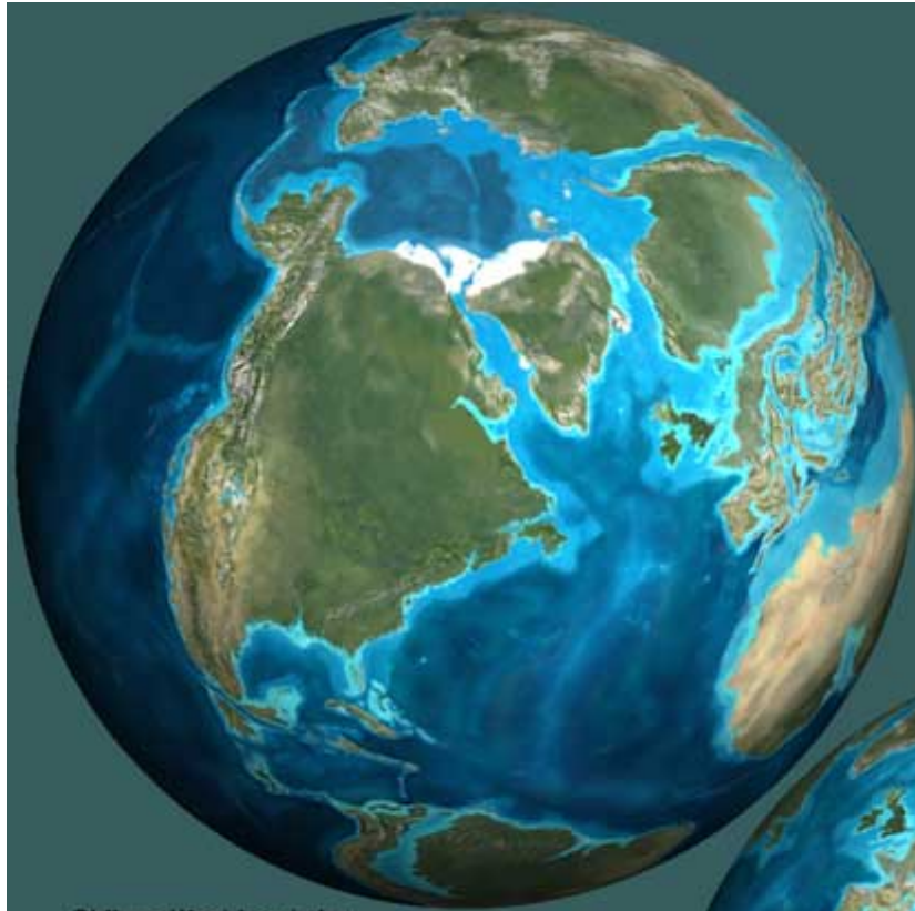
Oblique West-hemi view
