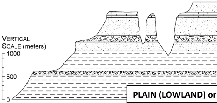
25 million years ago
