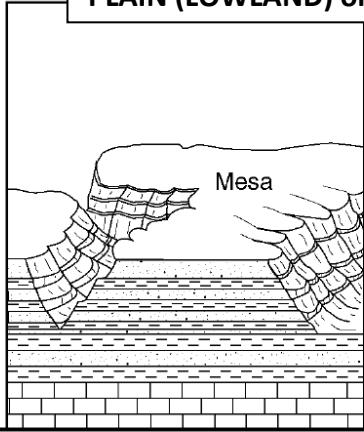
15 million years ago
