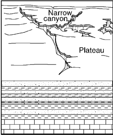
25 million years ago
